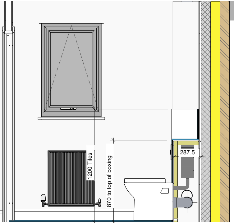
2 Bathroom - View B 1 : 25
