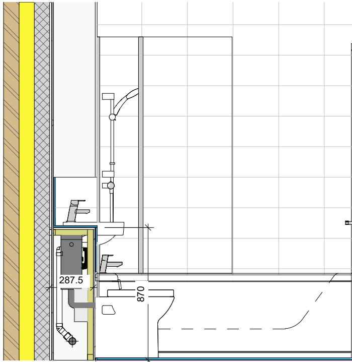
5 Bathroom - View D 1 : 25
