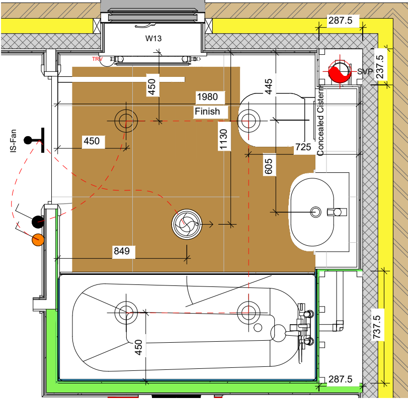
1 Bathroom Layout 1 : 25
