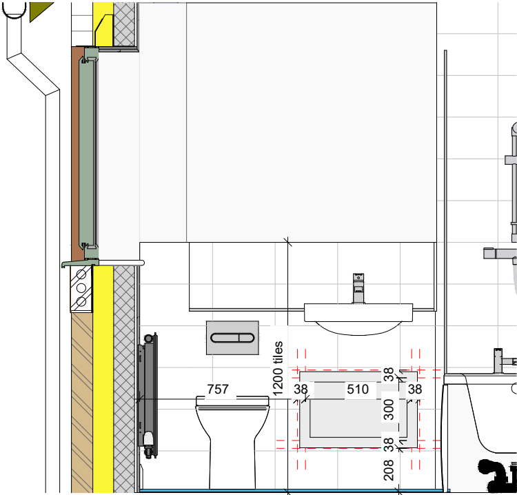
4 Bathroom - View C 1 : 25
